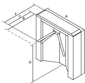
Trilock 75
